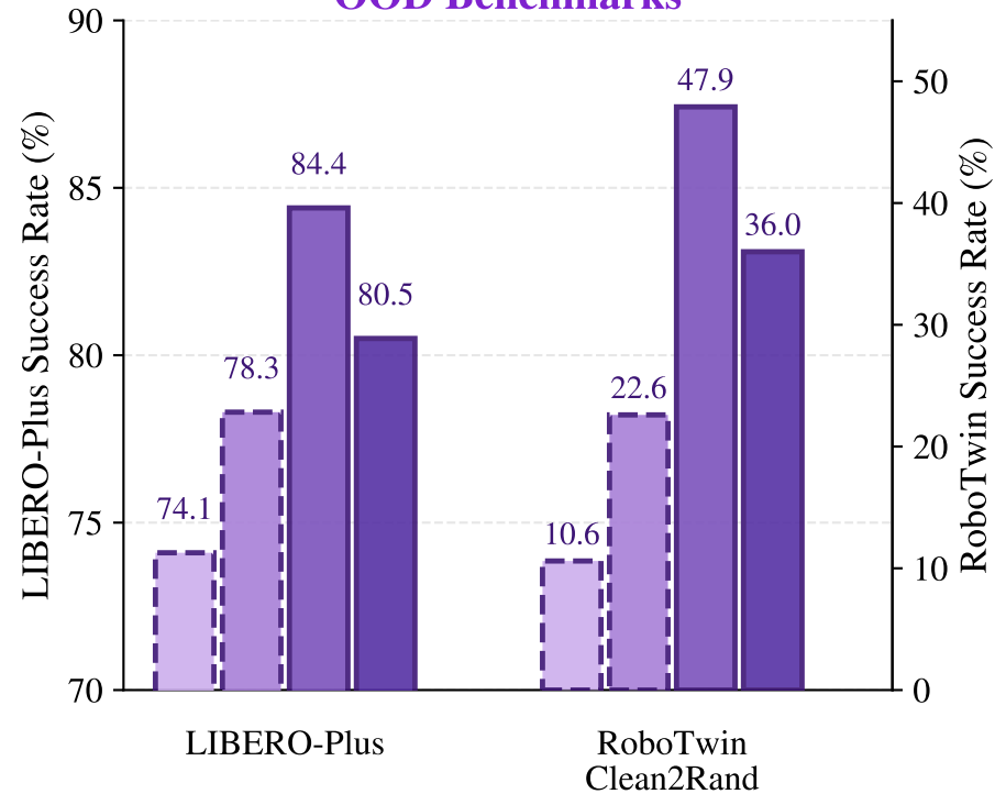
OOD Benchmarks
