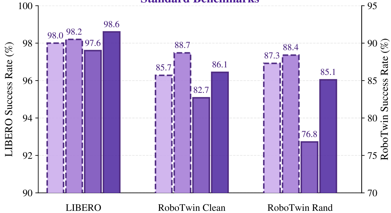
Standard Benchmarks
