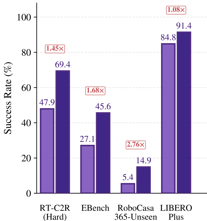
(a) Task & Scene Generalization
