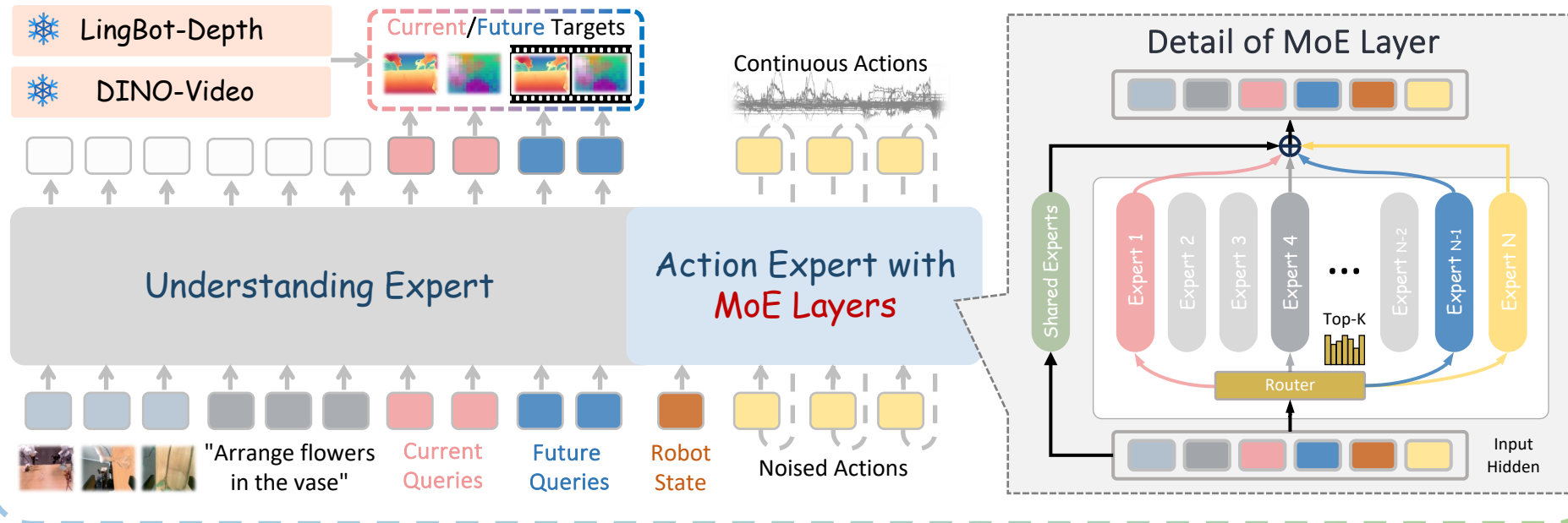
(a) Framework of LingBot-VLA 2.0
