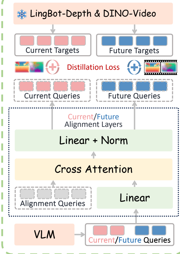
(b) Dual-Query Distillation
