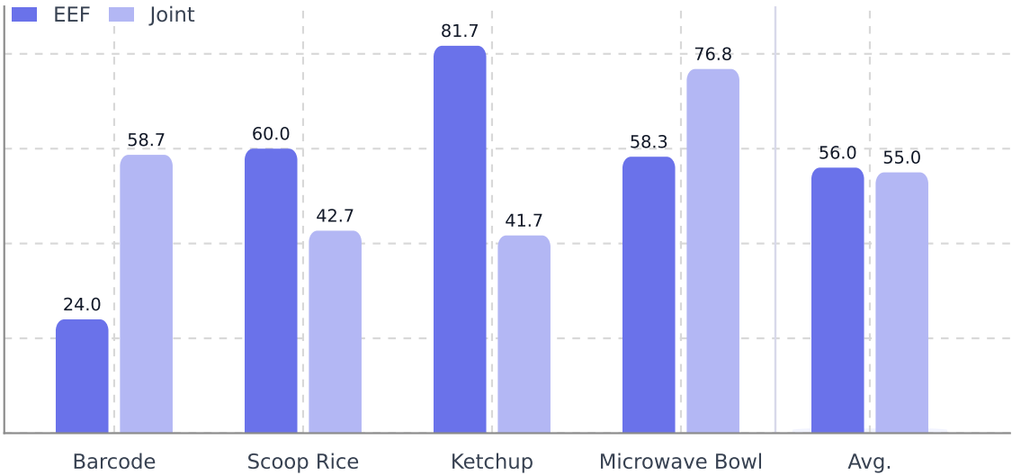
Action space
