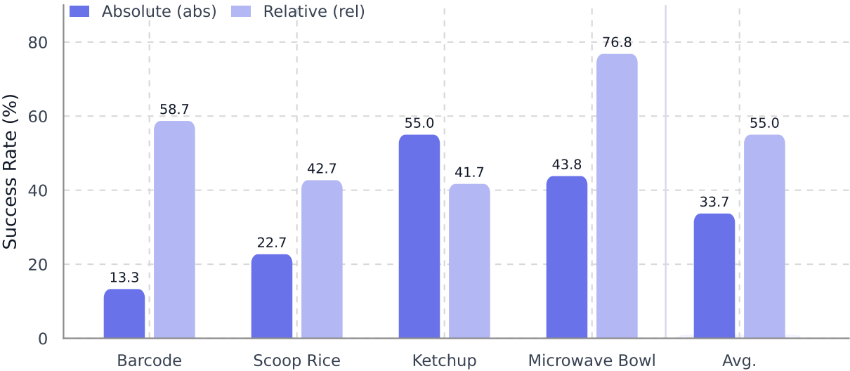
Action target
