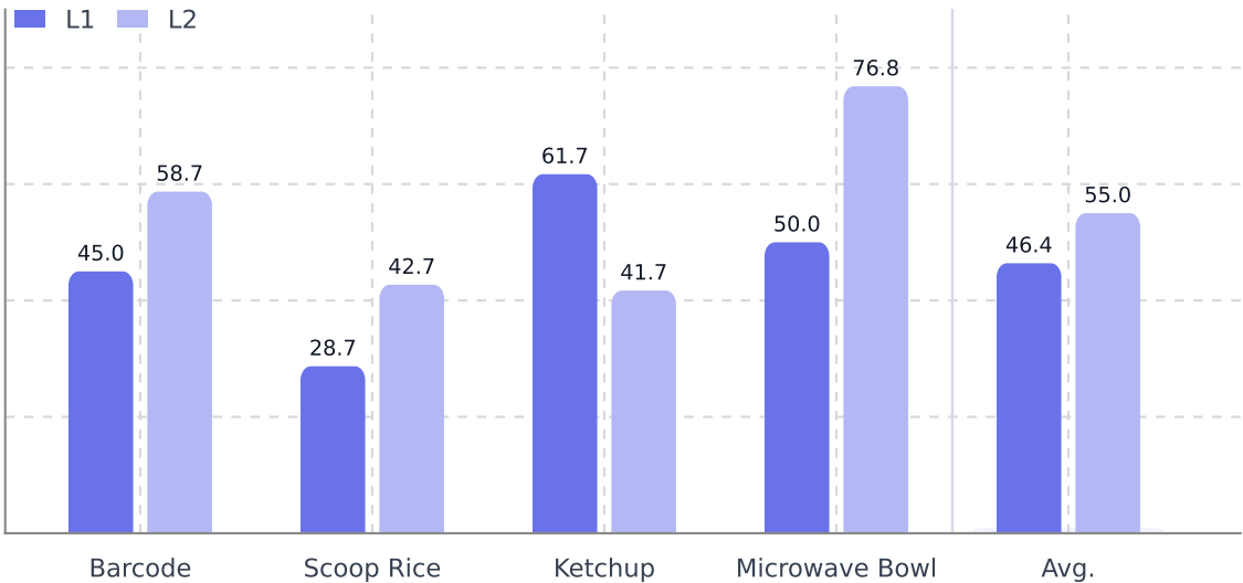
Loss
