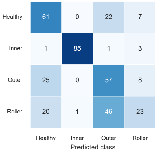
True class
