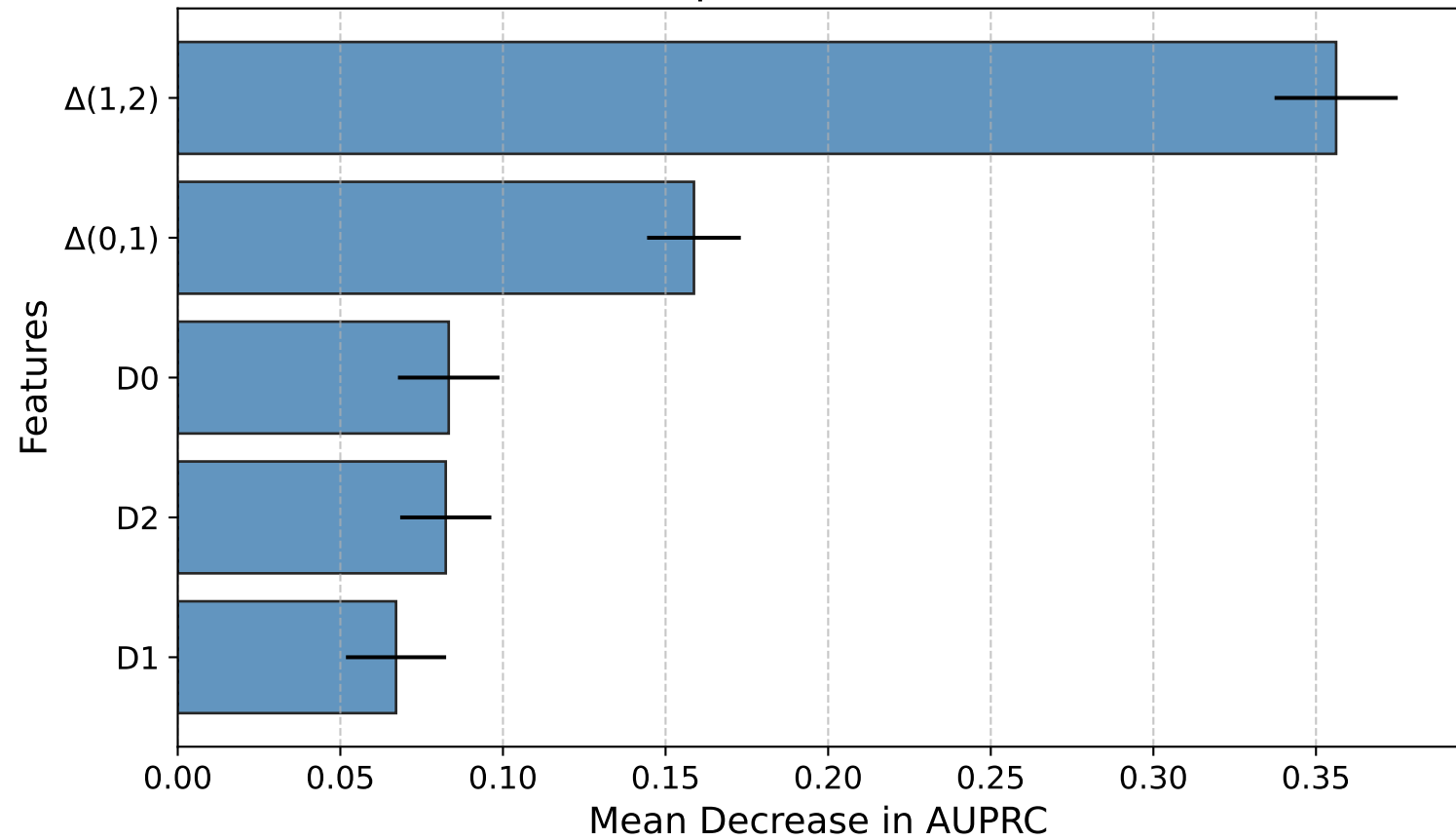
Permutation Feature Importance (SVM, RBF kernel, AUPRC)
