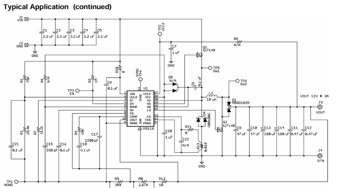
Figure 19. 12-V, 3-A Typical Application Schematic
