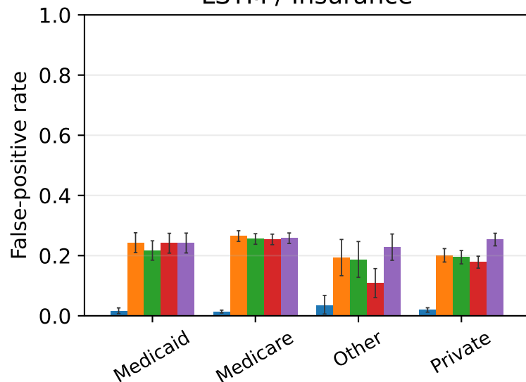
LSTM / Insurance
