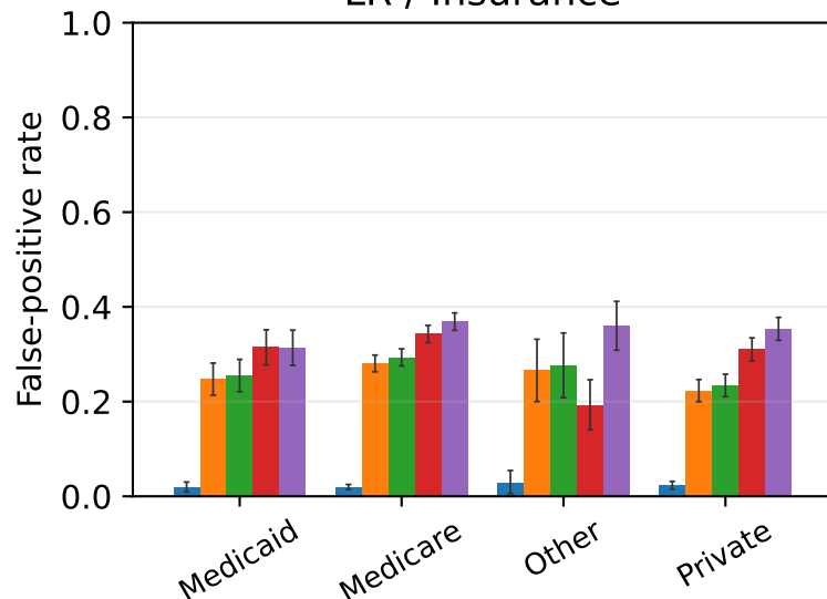
LR / Insurance
