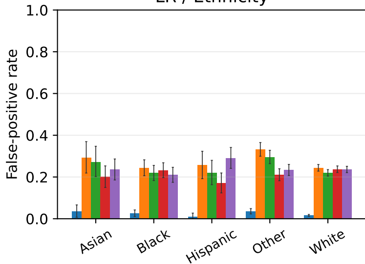
LR / Ethnicity
