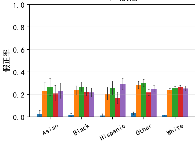
LSTM / 族裔
