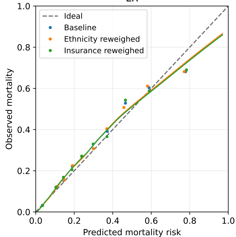
LR
