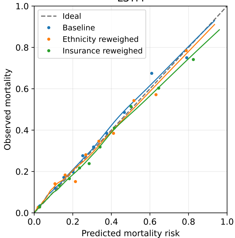
LSTM
