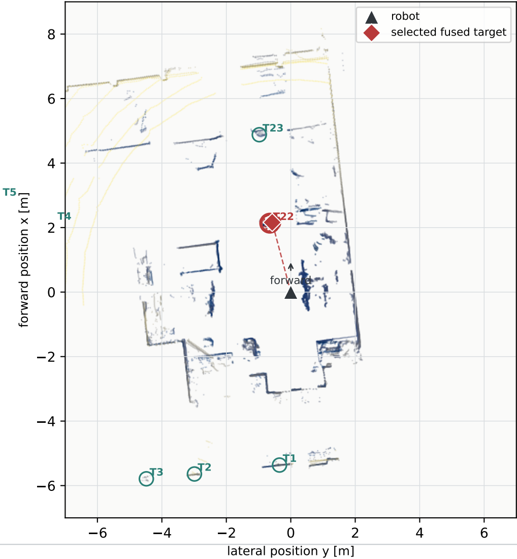
(b) LiDAR geometry and target-association state
