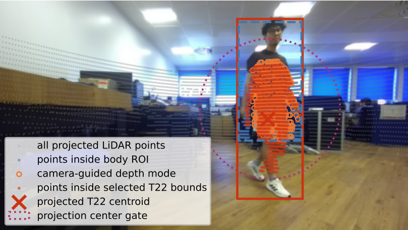
(b) Image-plane LiDAR association evidence
