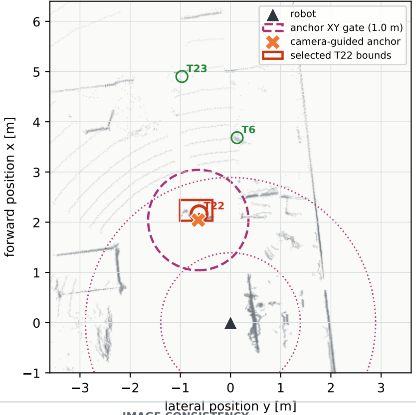
(c) Metric association gates in base frame
