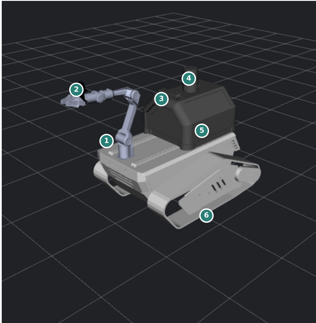
(a) Integrated mobile-manipulation digital model
