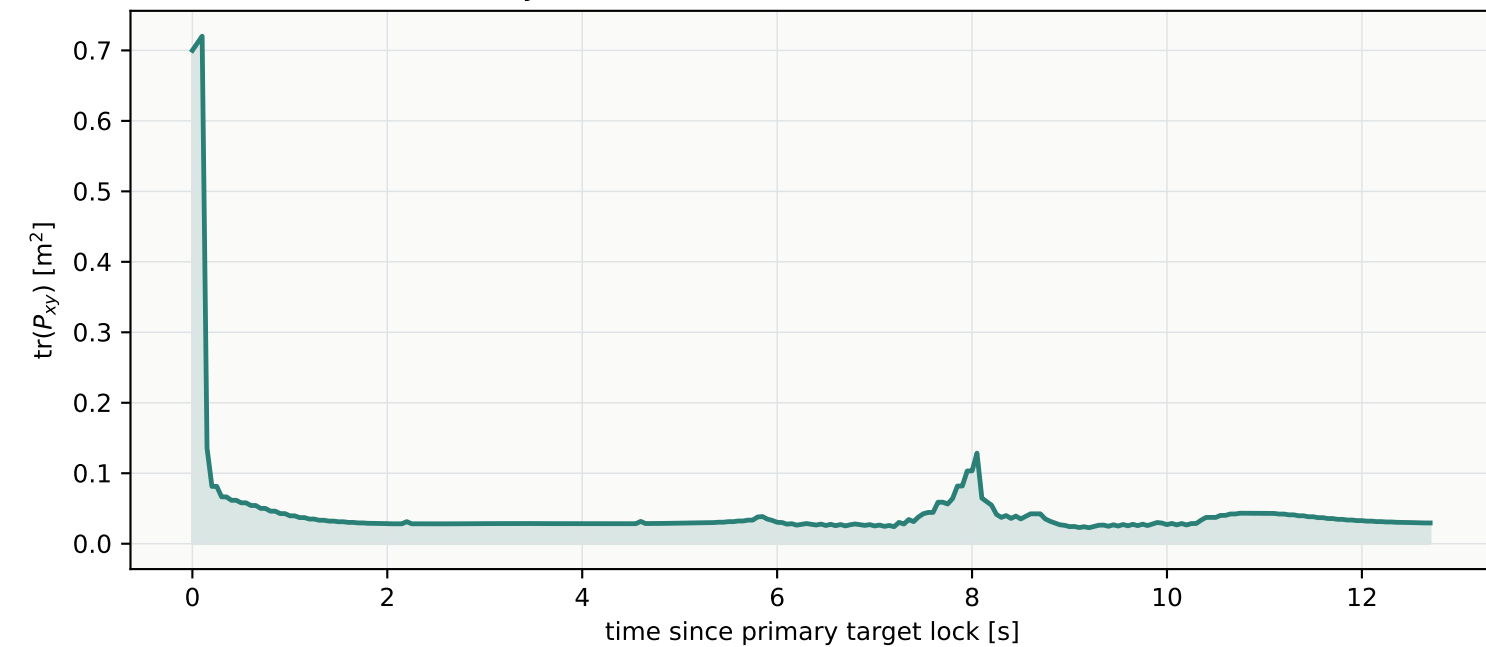
(c) Planar state uncertainty
