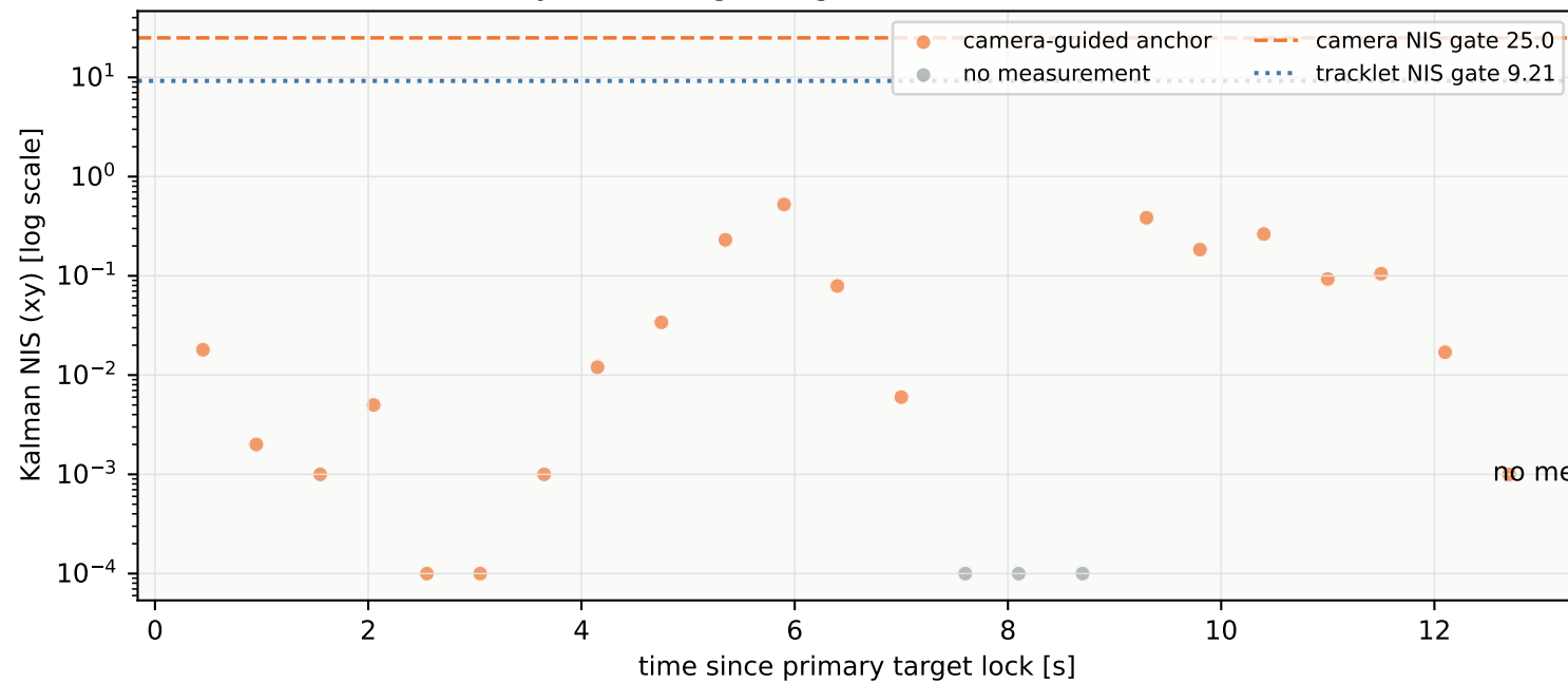
(a) Innovation consistency and configured gates
