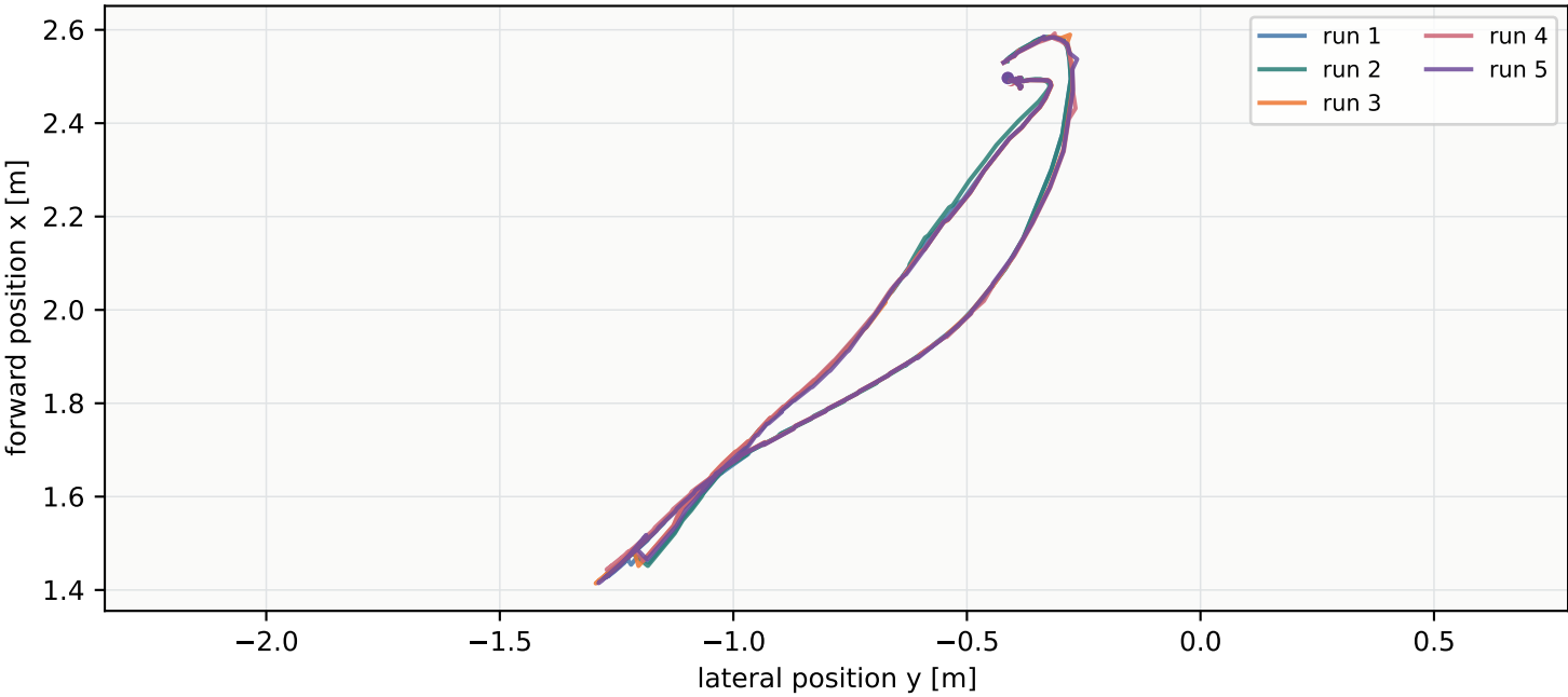
(a) Aligned physical target trajectories
