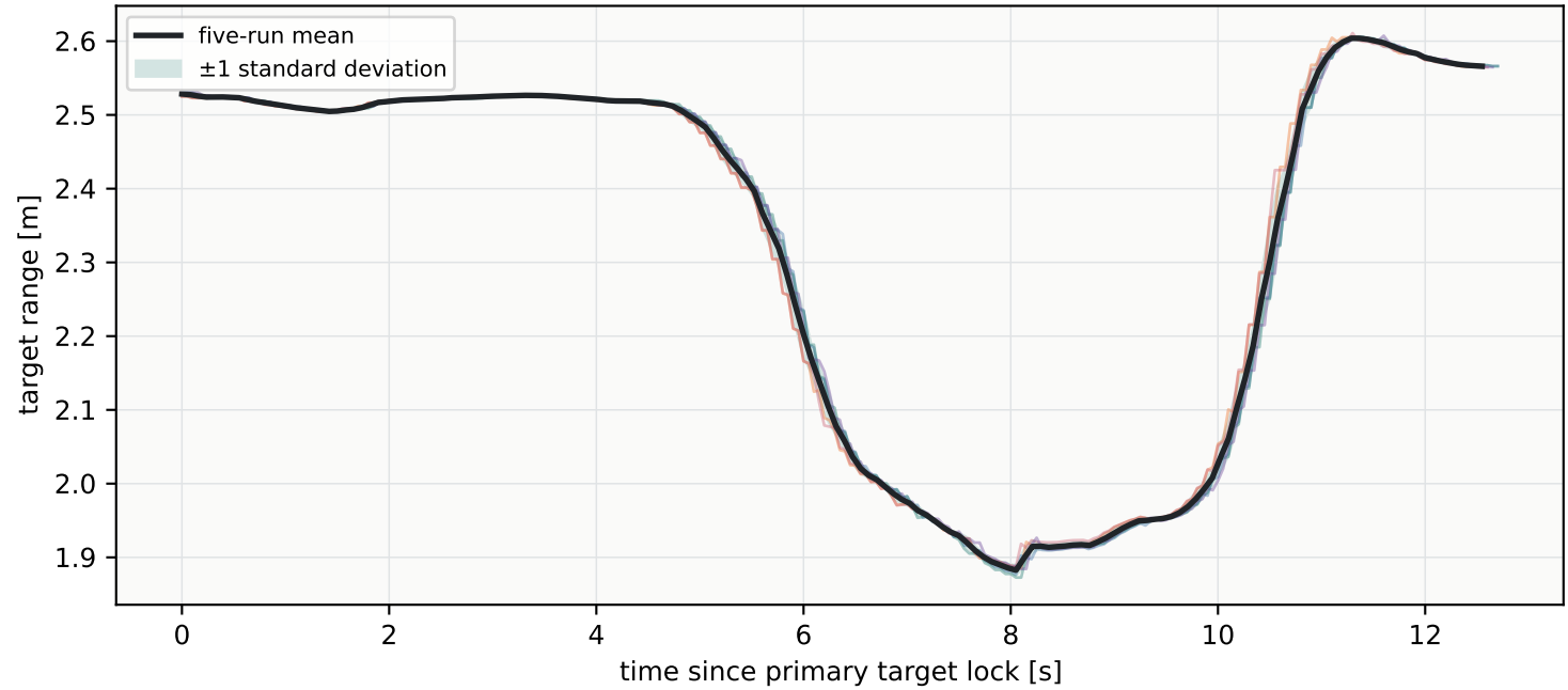
(b) Range repeatability
