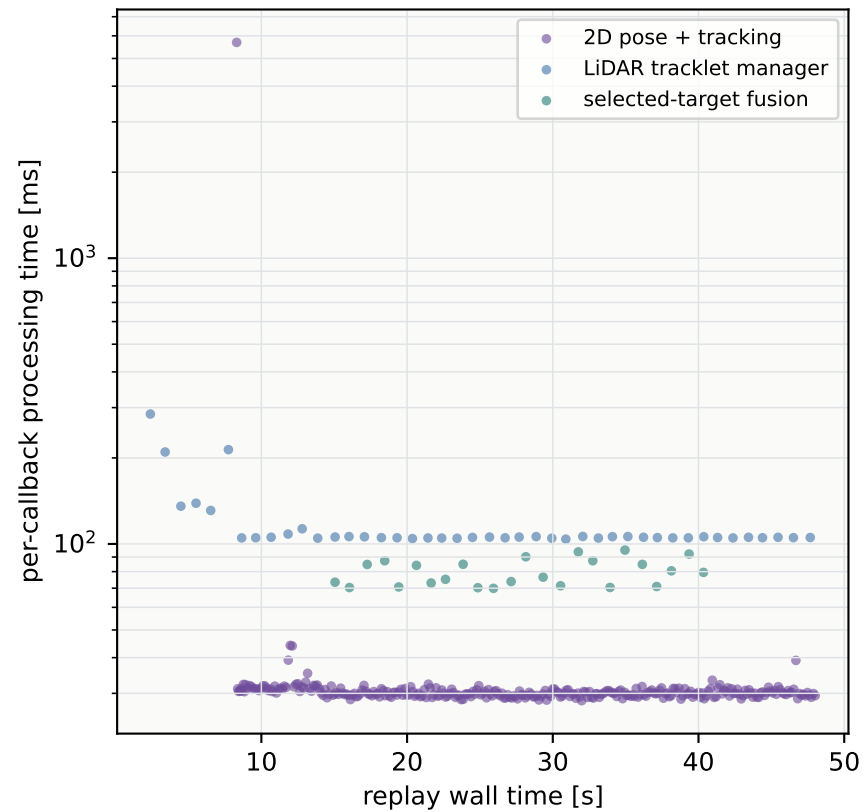
(a) Per-callback processing time
