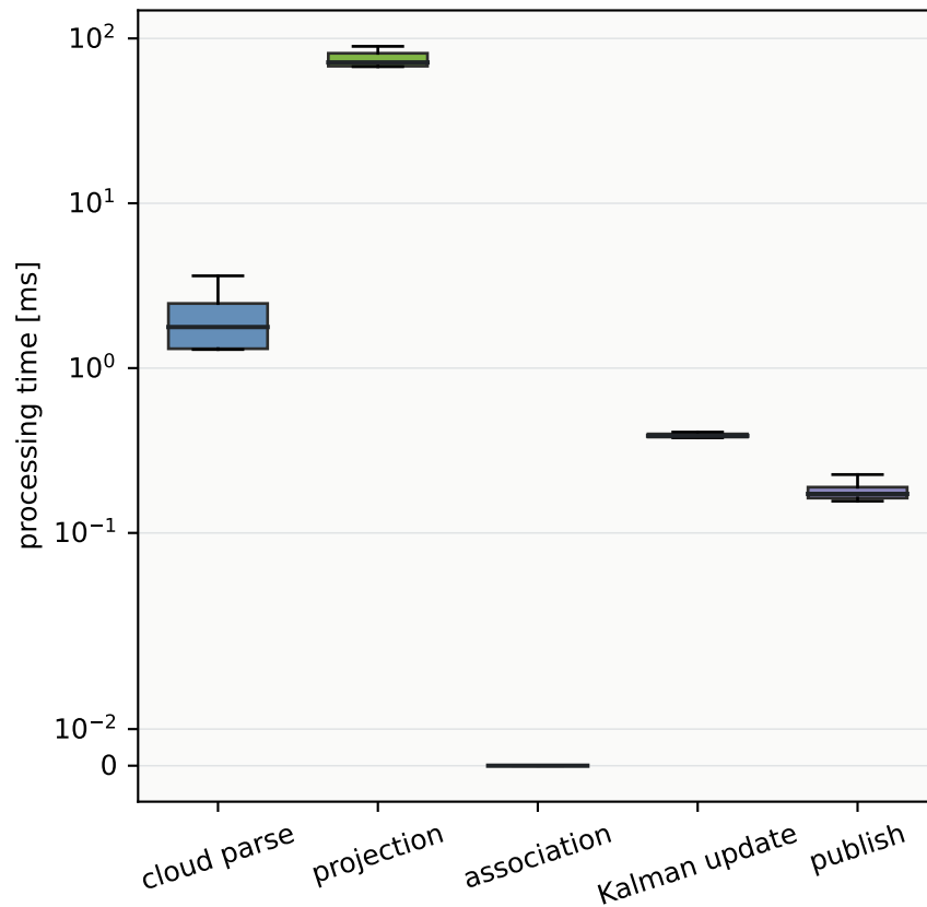
(b) Fusion-stage latency distribution
