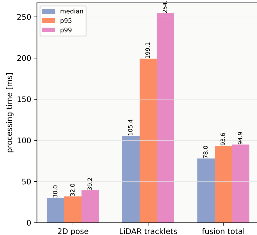
(c) Robust timing percentiles
