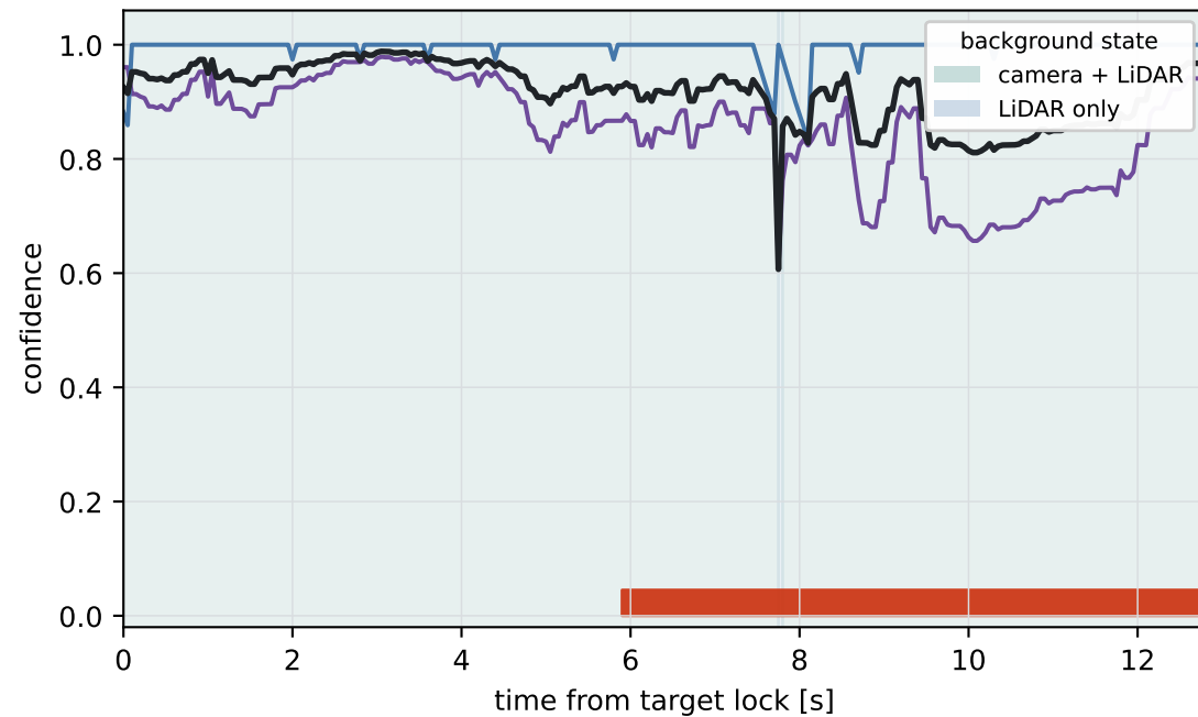
(c) Confidence and measurement-source continuity
