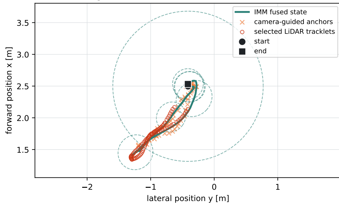
(a) Planar target-state estimation
