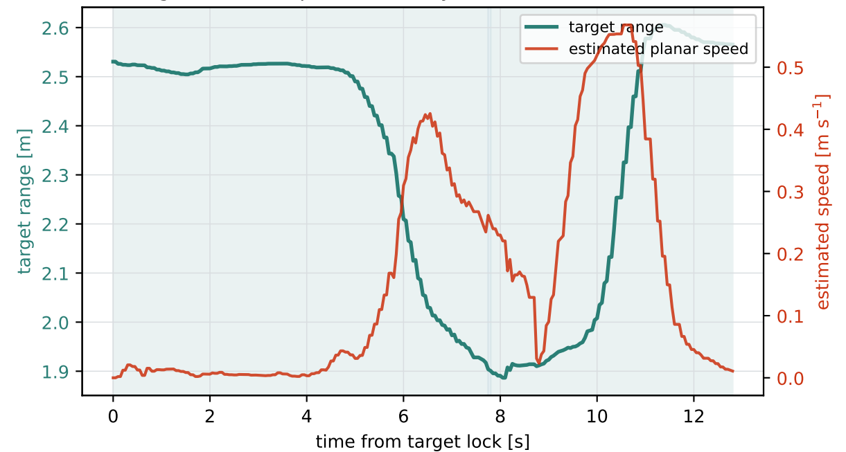
(b) Range and fused planar velocity
