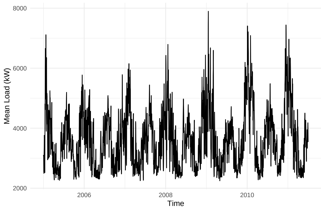
Daily Mean Electricity Load (2005–2011)
