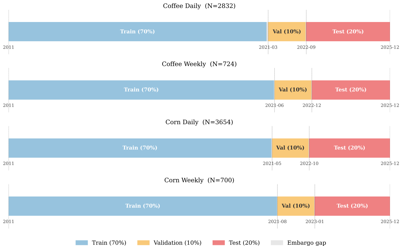
Fig. 3 — Temporal Train/Val/Test Split with Embargo Gaps
