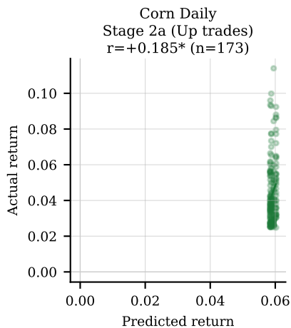
Fig. 5 — Hurdle Model: Predicted vs. Actual Return Magnitude
