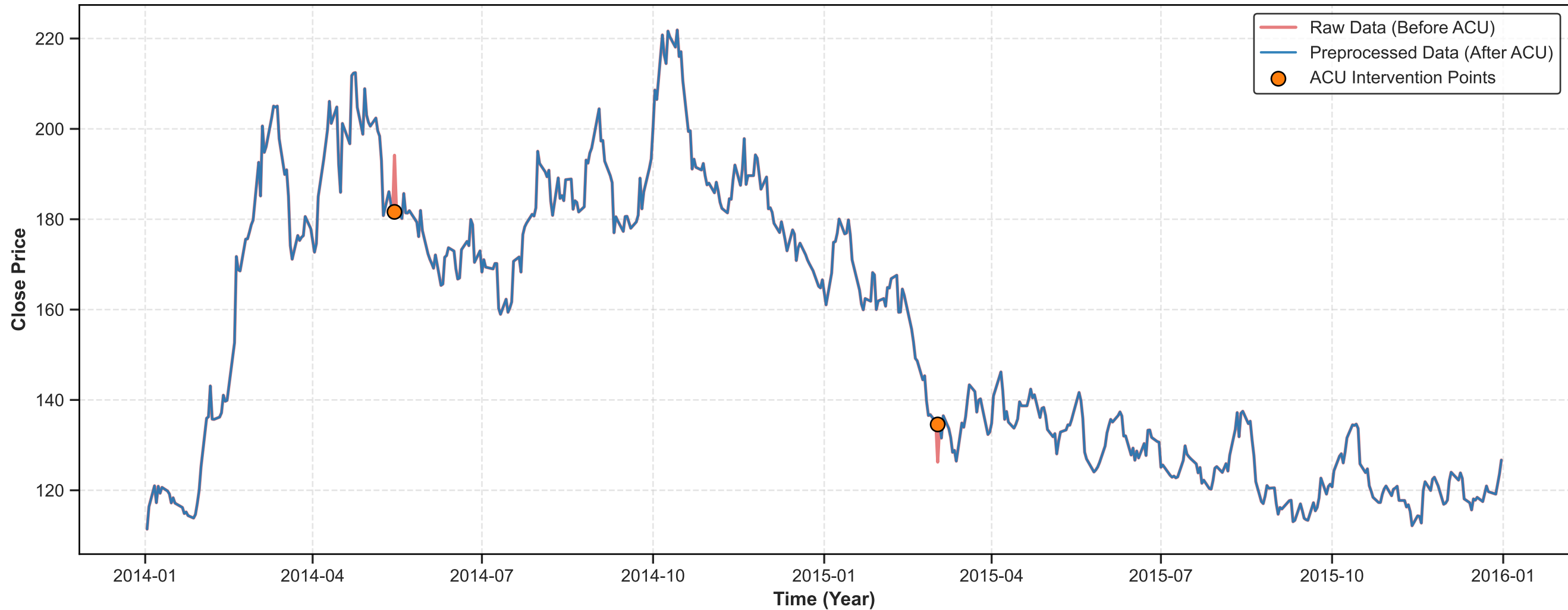
Fig. 3 — Comparison of Raw and ACU-Filtered Coffee Close Prices (2014-2016)
