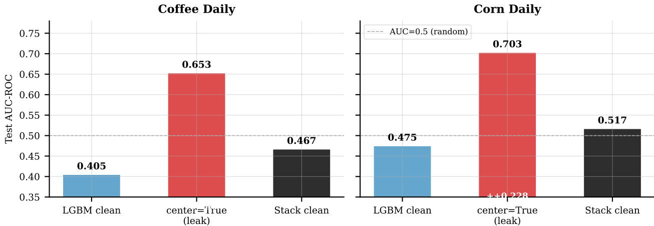
Fig. 7 — Ablation: Clean Pipeline vs Look-Ahead Leakage (center=True)
