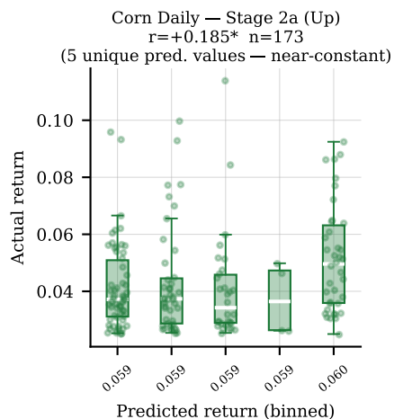
Fig. 8 — Hurdle Model: Stage 2a / Stage 2b / Full Hurdle
