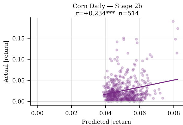
Fig. 5 — Hurdle Model: Stage 2b and Full Hurdle
