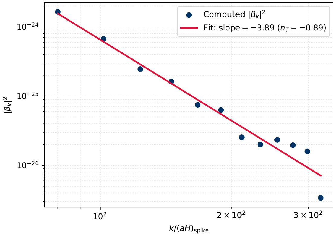
Computed tensor particle production (red tilt)
