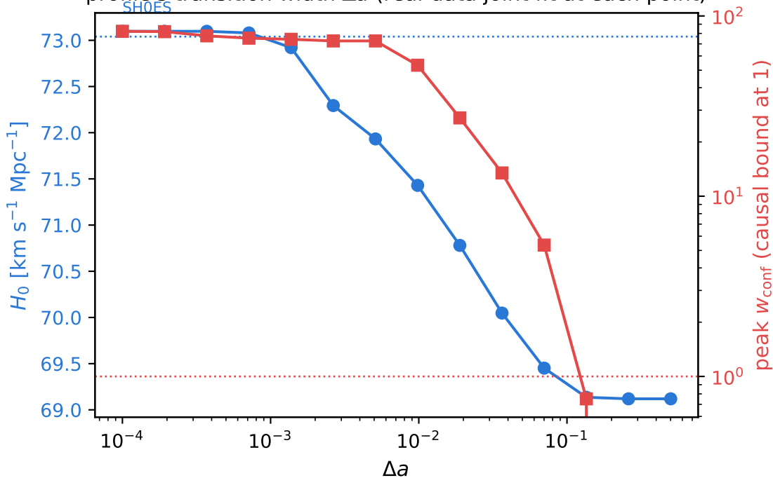
Tension relief versus causality across the confinement profile's transition width \Delta a (real-data joint fit at each point)
