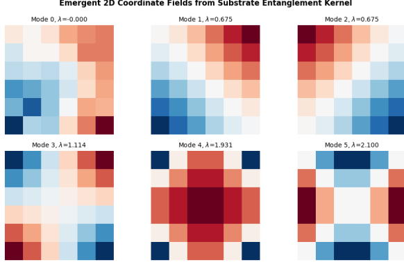
FIG. 1. Emergent 2D Eigenmodes from the Substrate Entanglement Kernel. Mode 0 ( \lambda = 0.000 ) tracks the invariant global ground state. Modes 1 and 2 exhibit an exact structural degeneracy ( \lambda = 0.675 ), manifesting as linear, mutually orthogonal spatial gradients that function as coordinate charts (x, y) over an isotropic 2D manifold. Higher modes define localized geometric harmonics with a natural UV pixelation cutoff.
