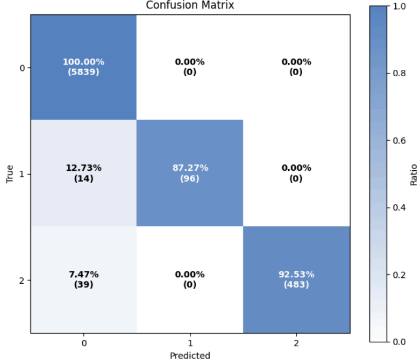
Figure 4: Confusion matrix for ST Elevation/Depression recognition.
