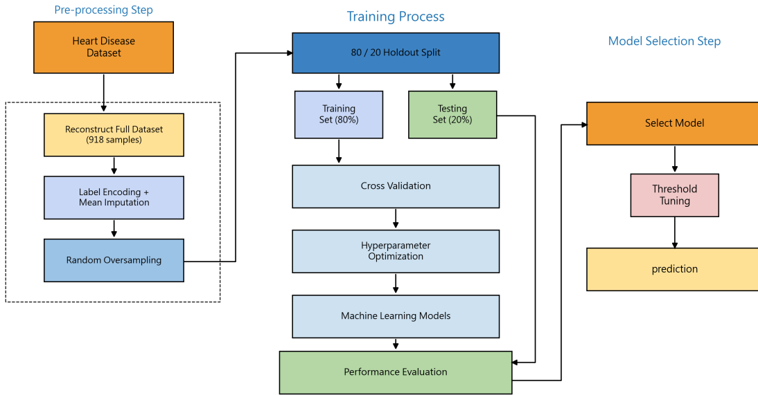
Figure 6: Flowchart of Model Development and Training
