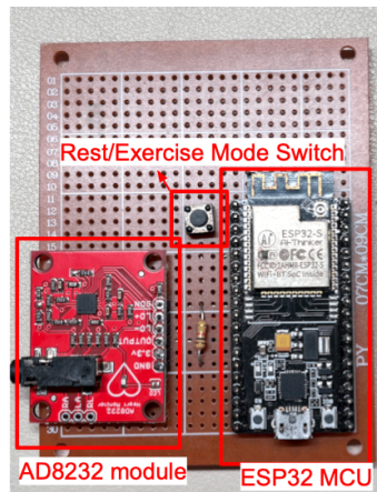
Figure 12: Hardware Implementation of the Wearable ECG Monitoring System
