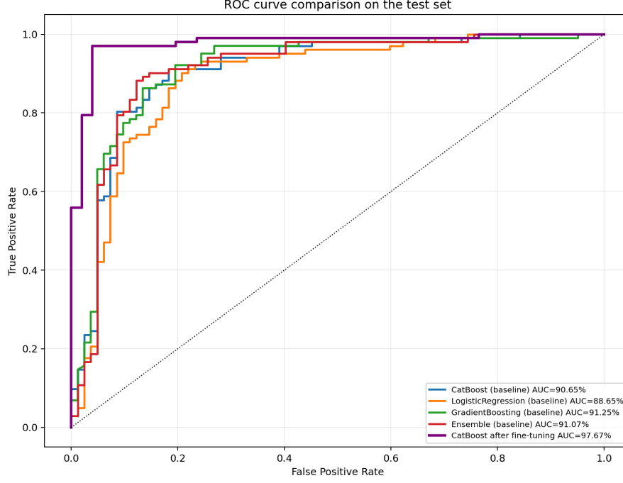
Figure 14: ROC curve comparison on test set
