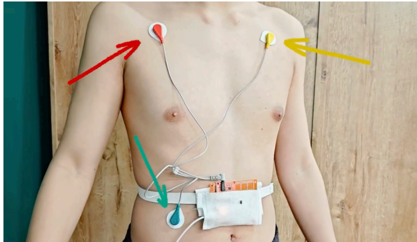
Figure 11: Wearable ECG System Configuration and Electrode Placement
