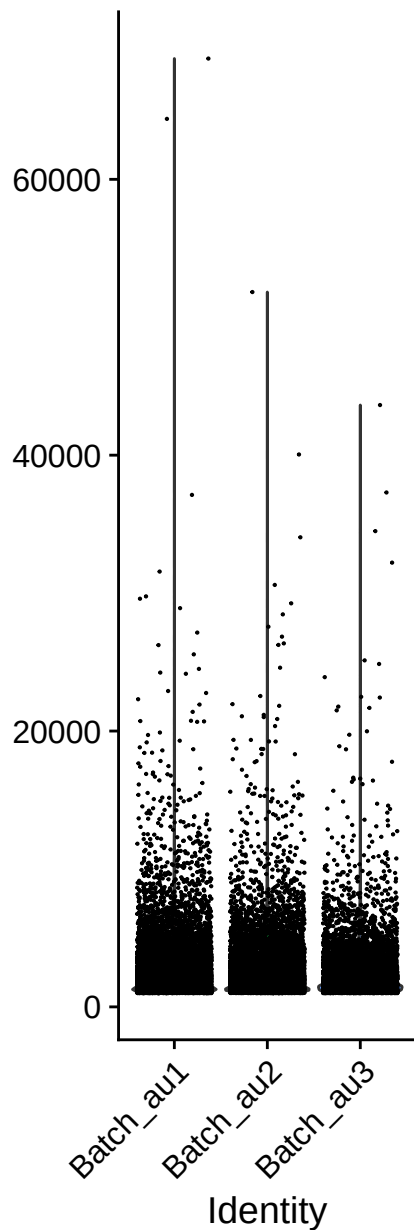
nCount_RNA
