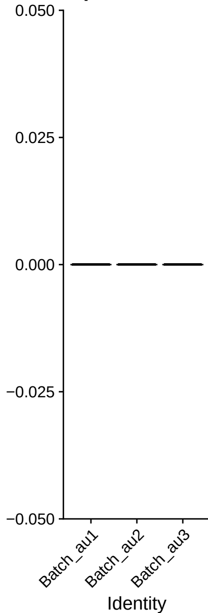
percent.mt
