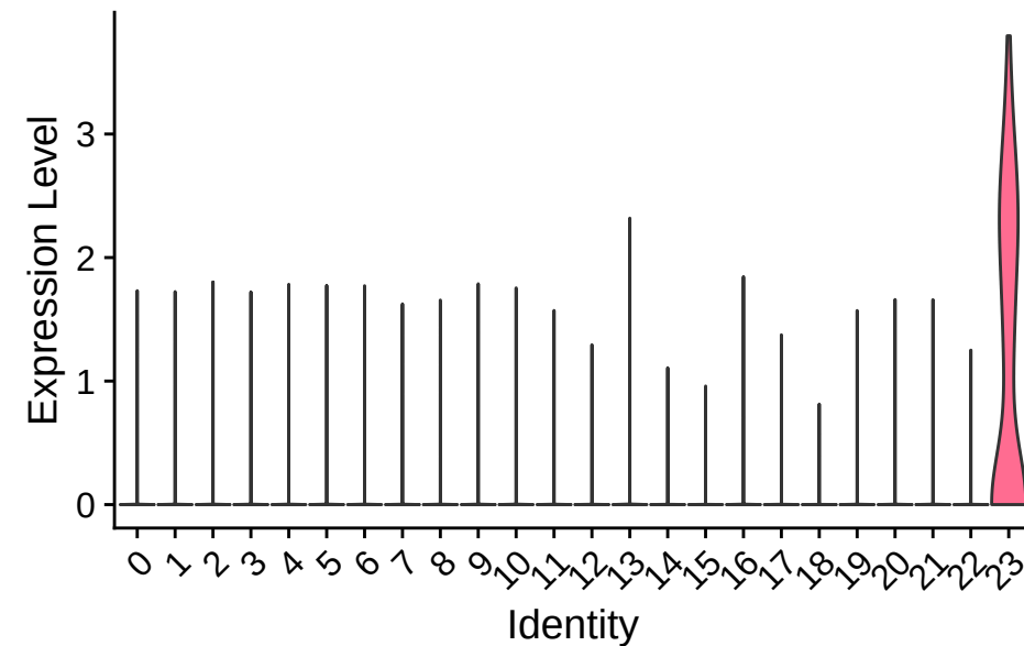
XLOC-006327#CEL2A-RAT#P00774
