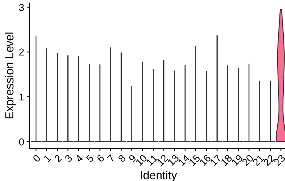
XLOC-000359#SVEP1-MOUSE#A2AVA0
