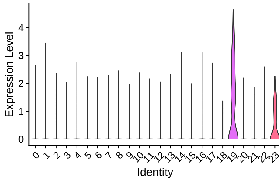
XLOC-000359#SVEP1-MOUSE#A2AVA0
