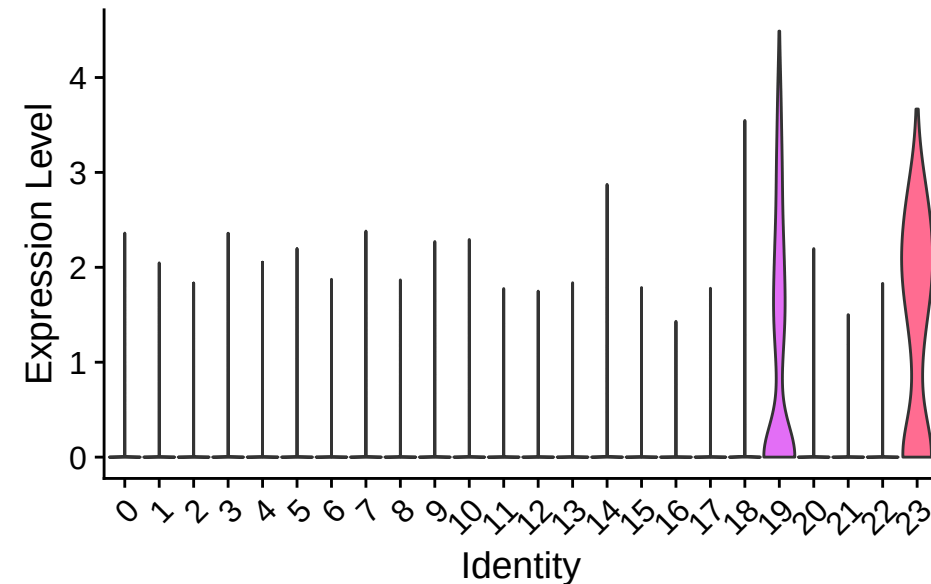
XLOC-006327#CEL2A-RAT#P00774
