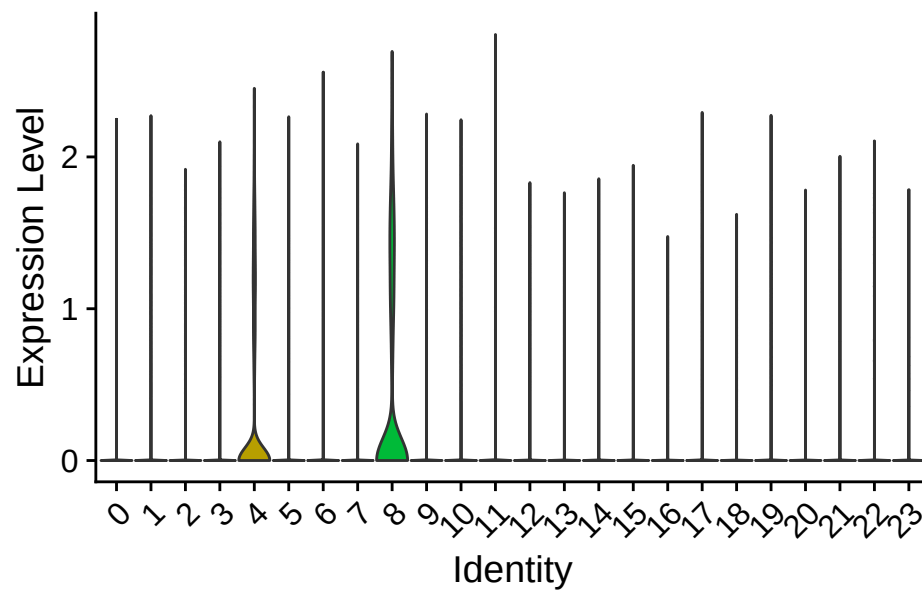
gene-evm.model.ptg000012l.280#GORS2-HUMAN#Q9H8Y8
