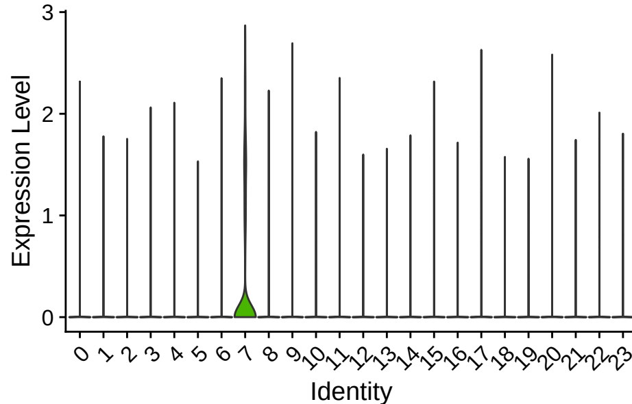
gene-evm.model.ptg000013l.805#CAB32-DROME#P41044
