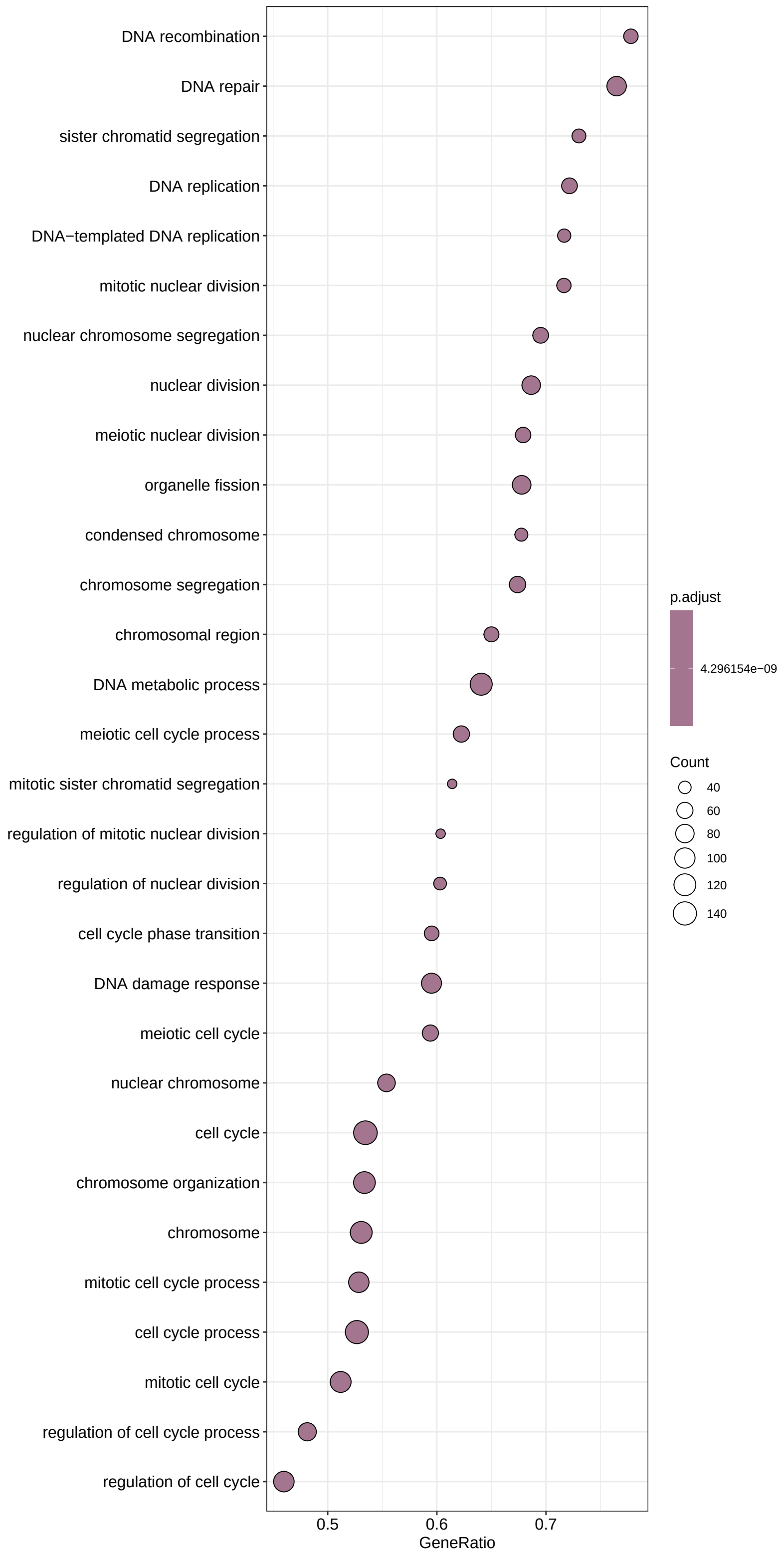
GSEA dotplot (cluster 10)
