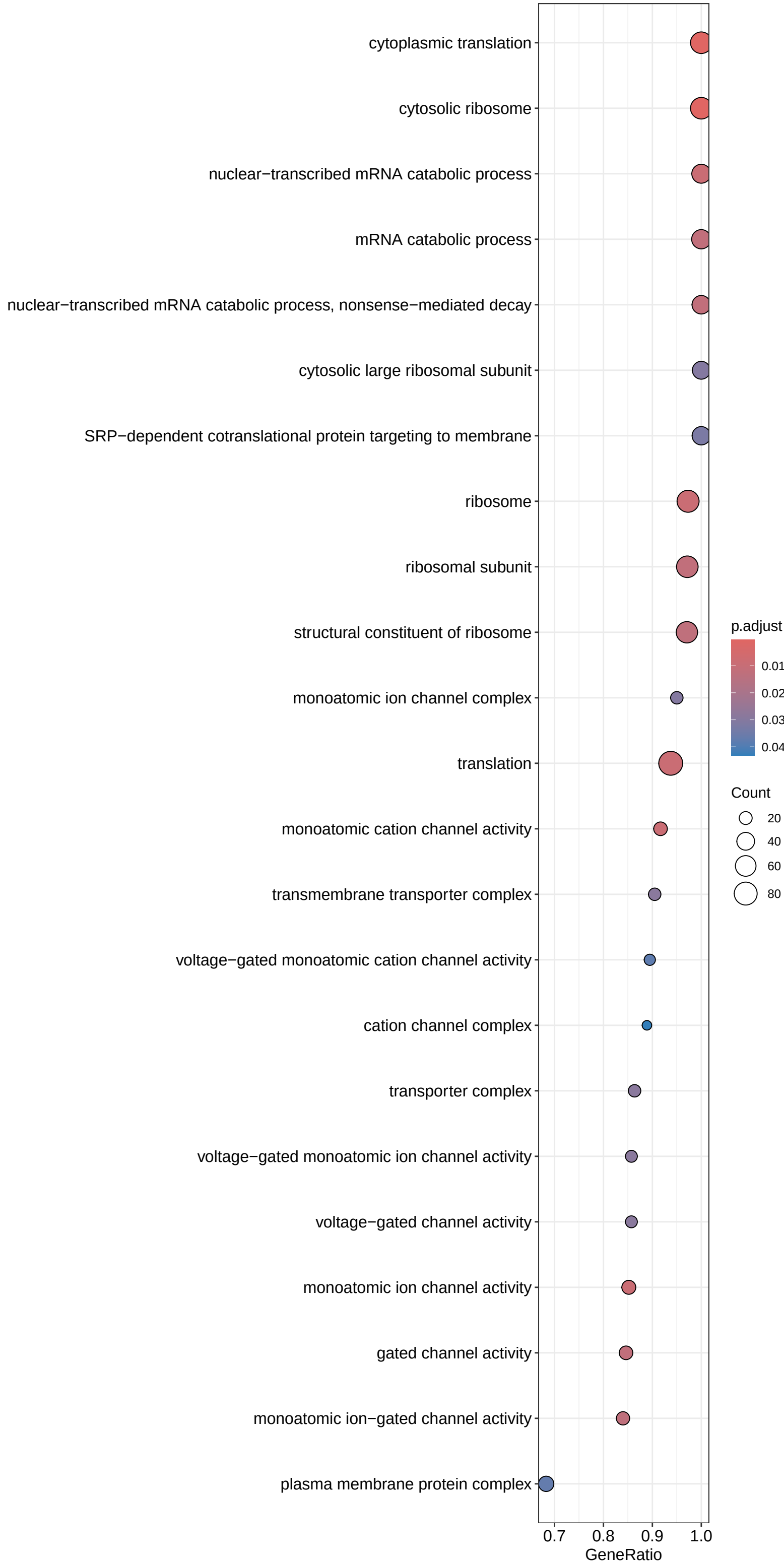
GSEA dotplot (cluster 15)
