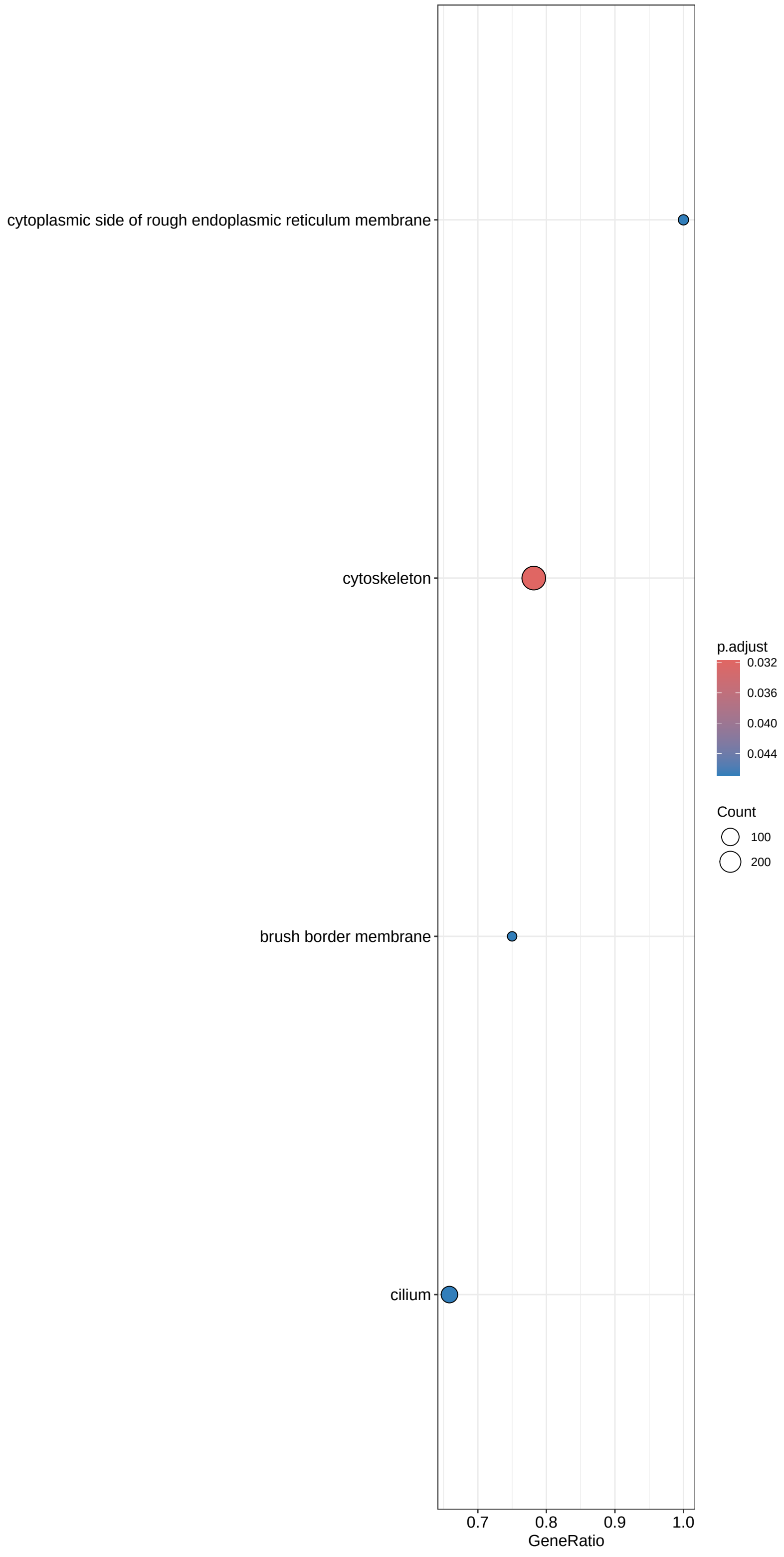
GSEA dotplot (cluster 16)
