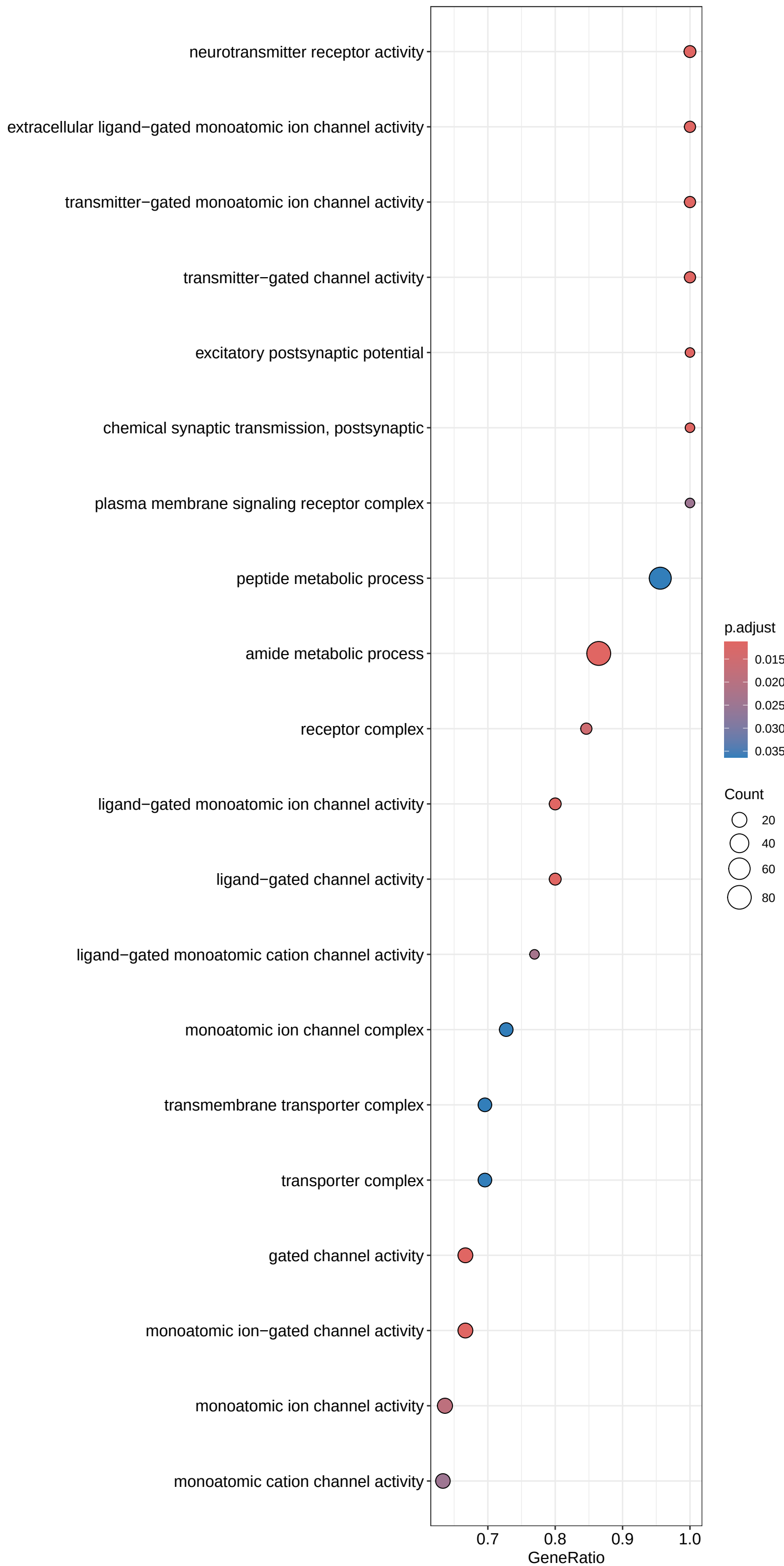
GSEA dotplot (cluster 9)
