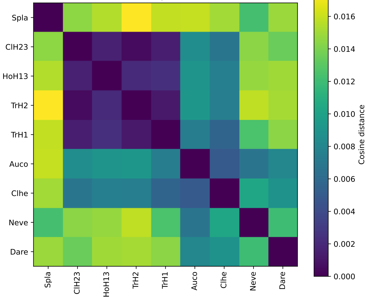
OG0000203 cross-species ESM2 distance
