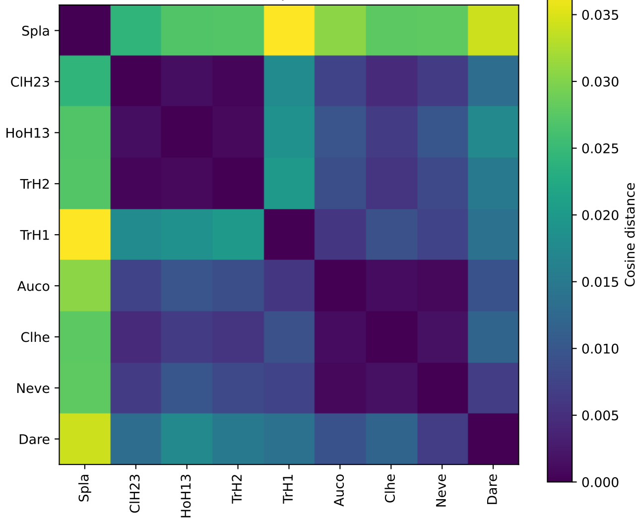
OG0000036 cross-species ESM2 distance
