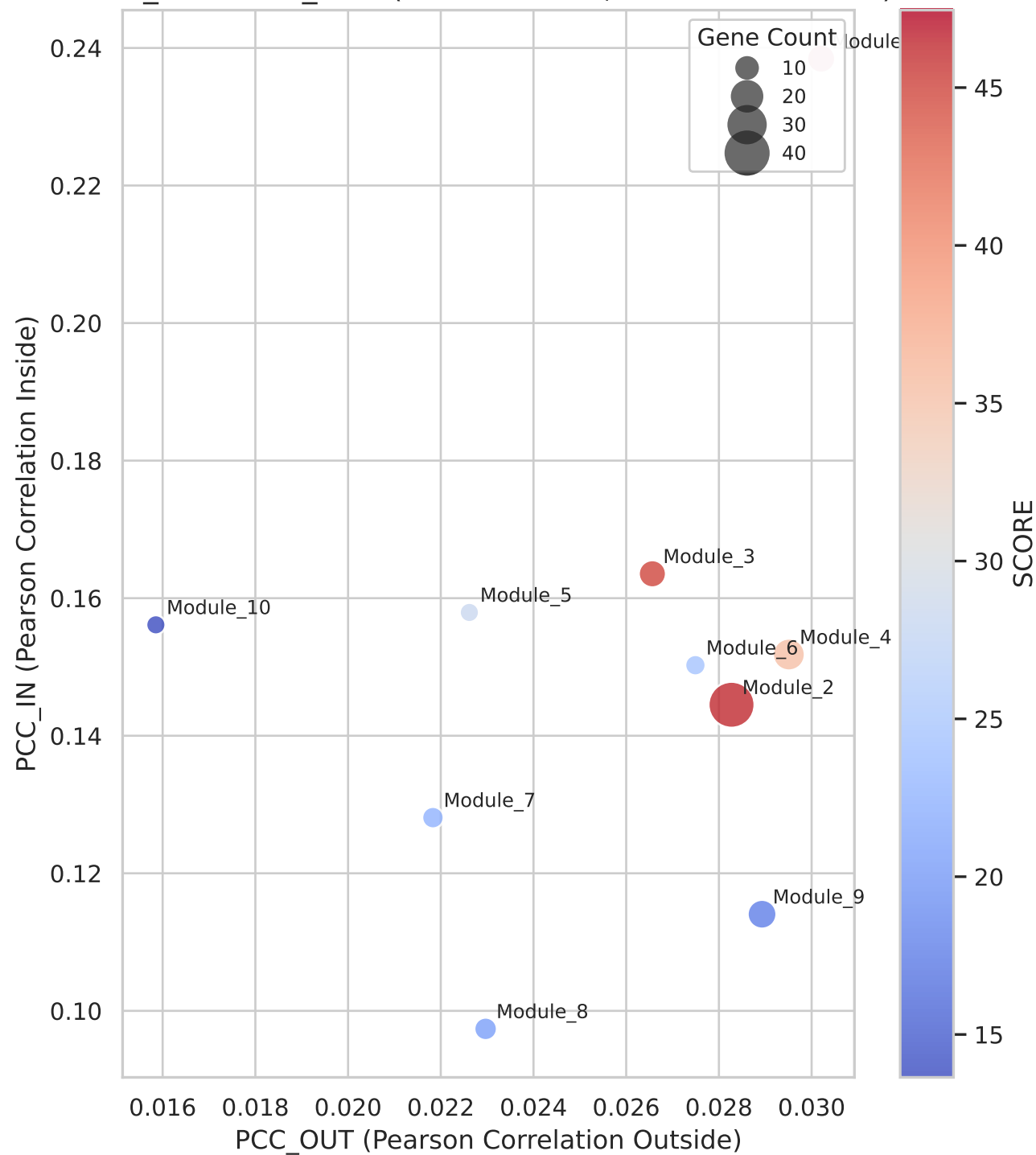
PCC_IN vs PCC_OUT (Color: SCORE, Size: Gene Count)
