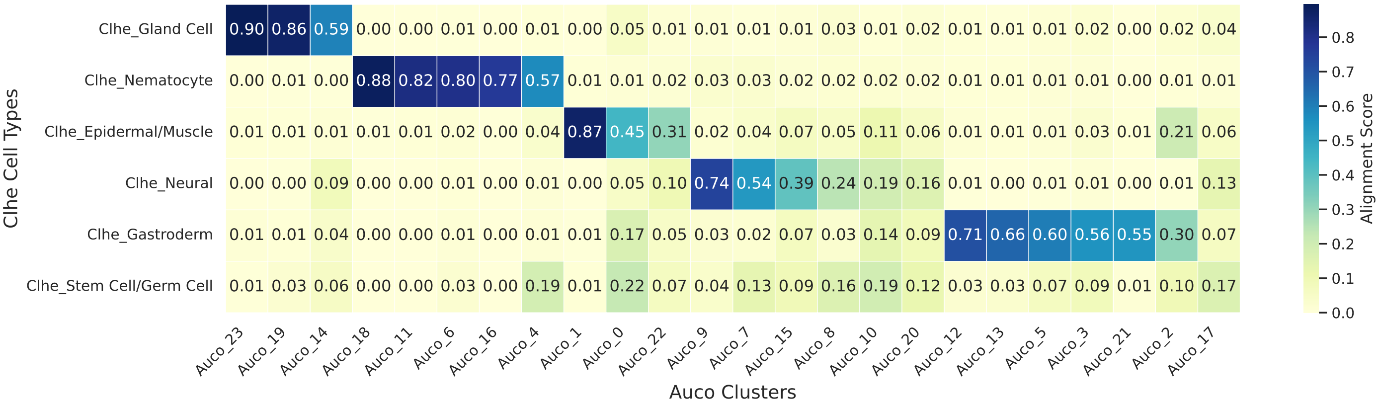
SAMap Mapping (Clhe-Auco)
