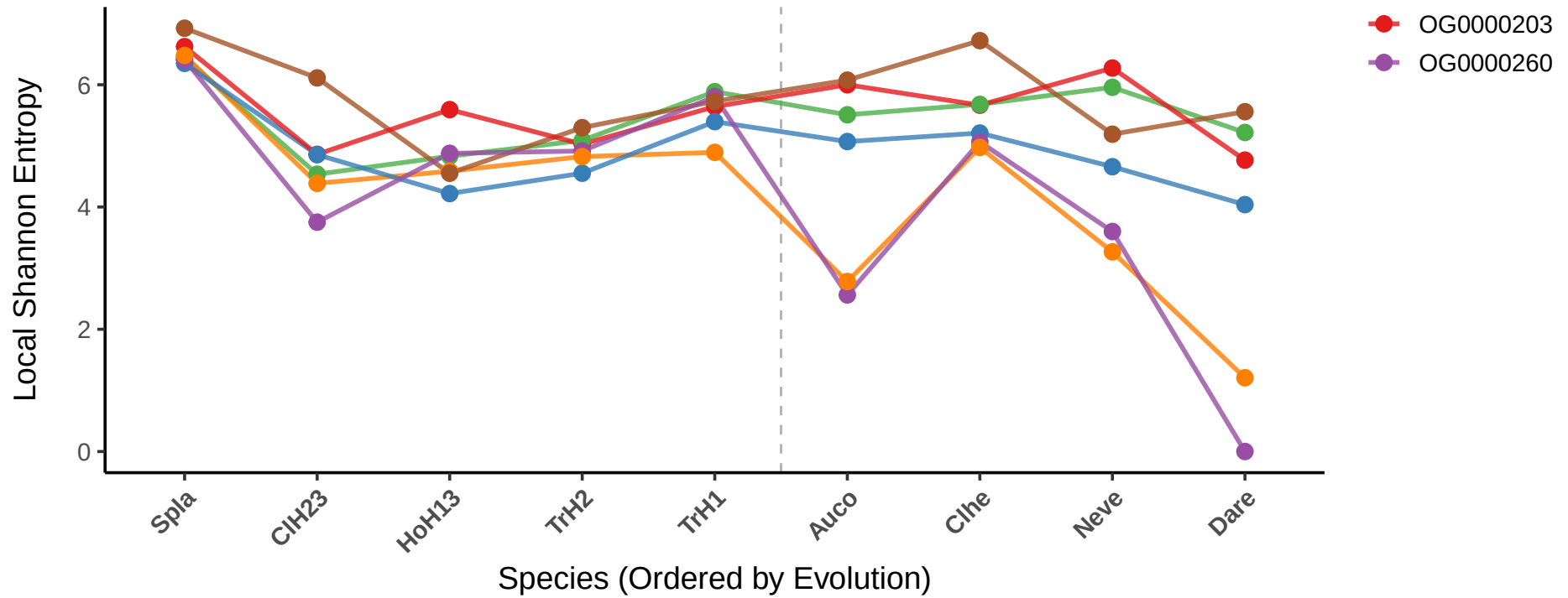
Local Entropy Complexity Trajectory
