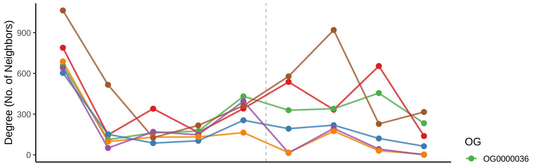
Network Degree Connectivity Trajectory
