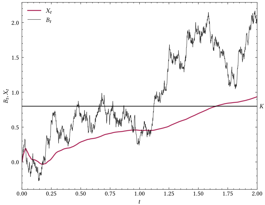
Figure 3: Brownian motion B_t and its moving average X_t
