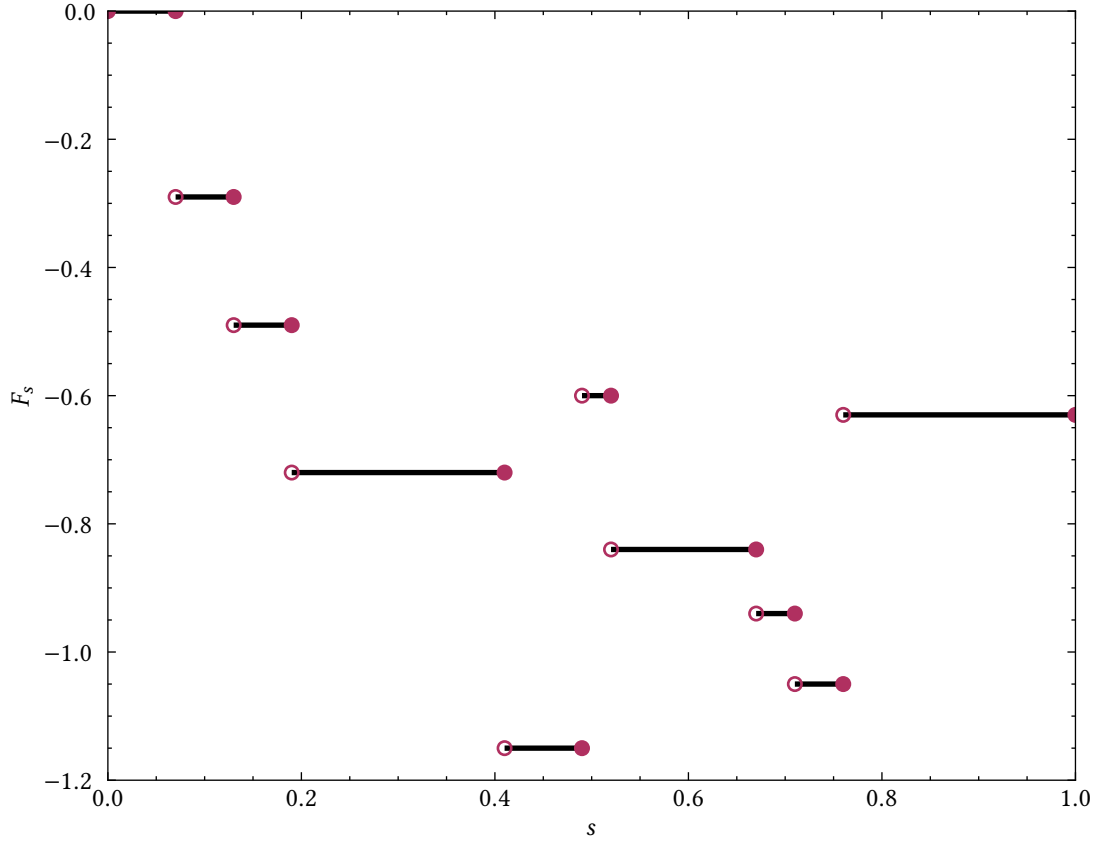
Figure 1: A realisation of a simple process.
