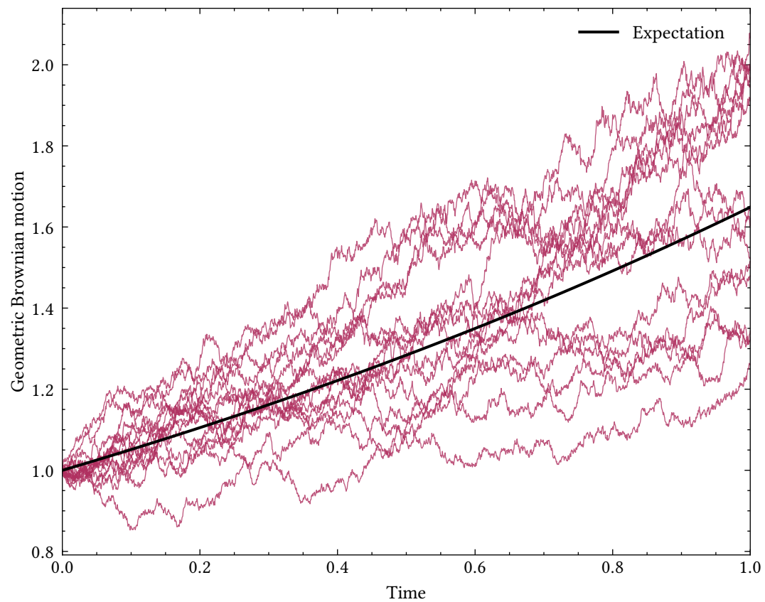
Figure 2: Geometric Brownian motion sample path and expectation for \mu = 0.5 , \sigma = 0.2 and S_0 = 1 .
