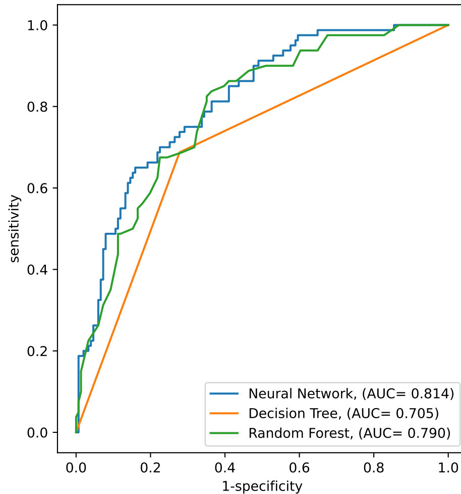
ROC curve test
