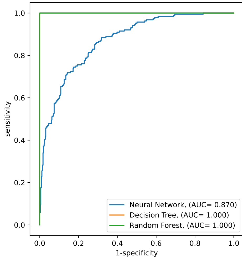
ROC curve train
