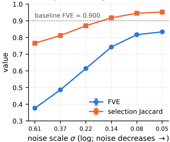
TopK: FVE and Jaccard vs. \sigma
