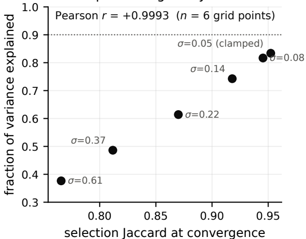
TopK: FVE against Jaccard
