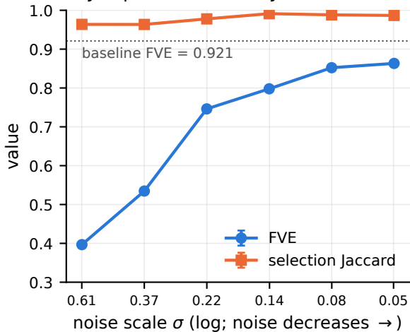
JumpReLU: FVE and Jaccard vs. \sigma
