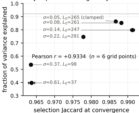
JumpReLU: FVE against Jaccard
