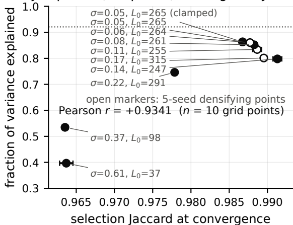
JumpReLU (ten points): FVE against Jaccard
