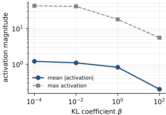
Activation scale collapses with \beta
