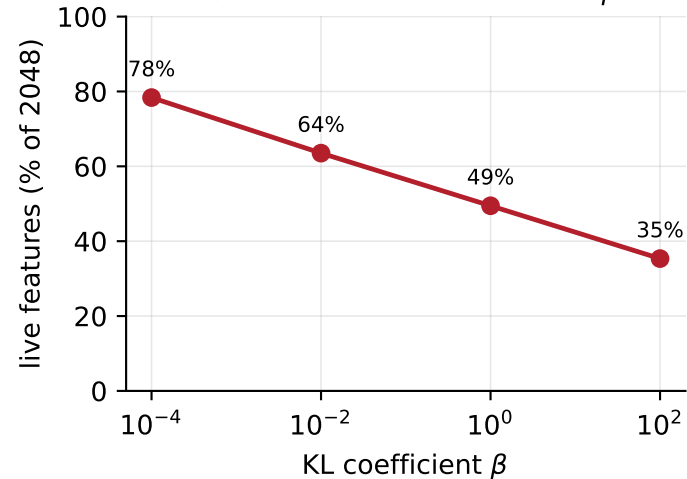
Feature death is monotonic in \beta
