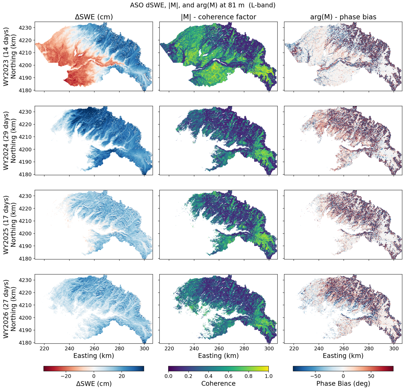
Figure 4. Lidar-derived \Delta\text{SWE} , sub-window coherence factor |M| , and retrieval bias \arg(M) at 81 m for the four Tuolumne lidar pairs (rows, labeled by water year and temporal baseline), evaluated at L-band, 40^\circ local incidence angle. Columns: the 81 m block-averaged \Delta\text{SWE} field ( left ), |M| ( center ), and \arg(M) ( right ).
