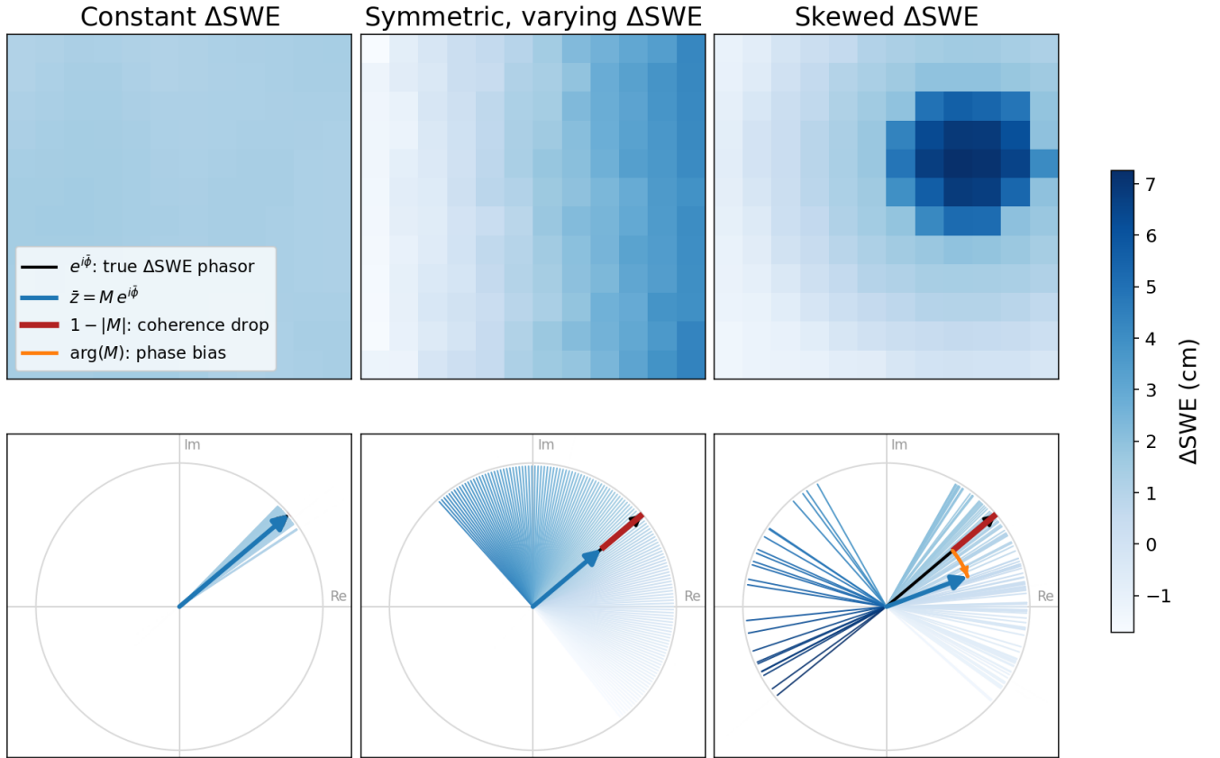
Figure 1. Sub-window \Delta\text{SWE} variability and its effect on the multi-looked phasor (all other decorrelation removed). Top: \Delta\text{SWE} in one window (cm), constant (left), varying symmetrically (middle), and skewed (right). Bottom: per-cell unit phasors ( \phi = \kappa\Delta\text{SWE} , colored by \Delta\text{SWE} ). Black: mean phasor e^{i\bar{\phi}} ; blue: resultant \bar{z} = M e^{i\bar{\phi}} ; red: coherence loss 1 - |M| ; orange arc: retrieval bias \arg(M) .
