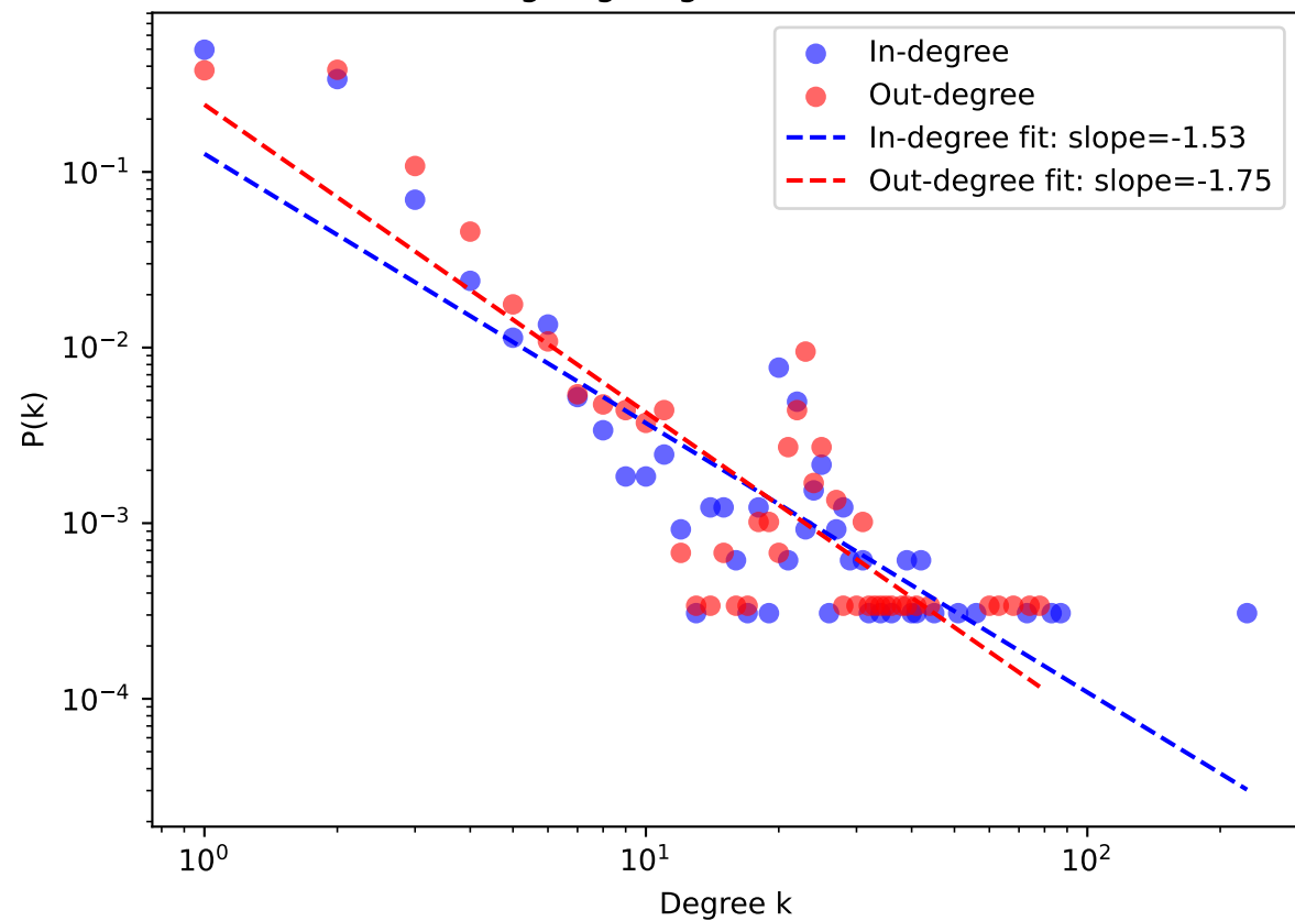
Log-Log Degree Distribution
