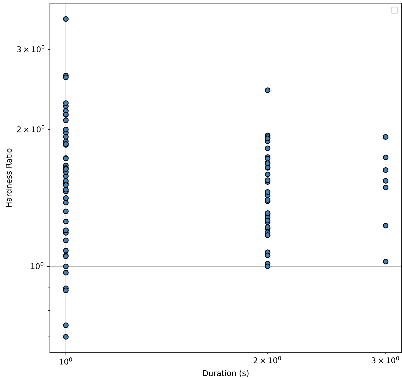
Duration and Hardness Ratio
